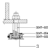
SECTION H-H
